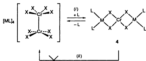
Scheme 6 (i) X = Me, OPh or OPr t , M = Na or Li, L = thf, Et 2 O or py; (ii) X = NR 2 , M = Li
