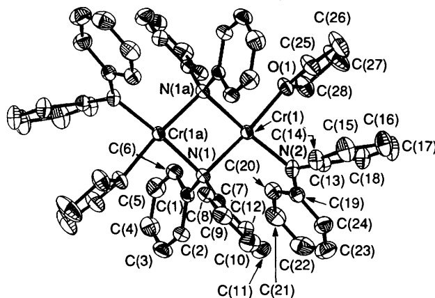
Fig. 2 An ORTEP plot of compound 2
